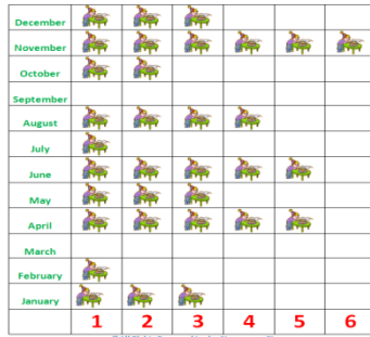
Birthday Graph
